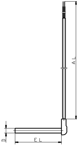
Type 902150/40
