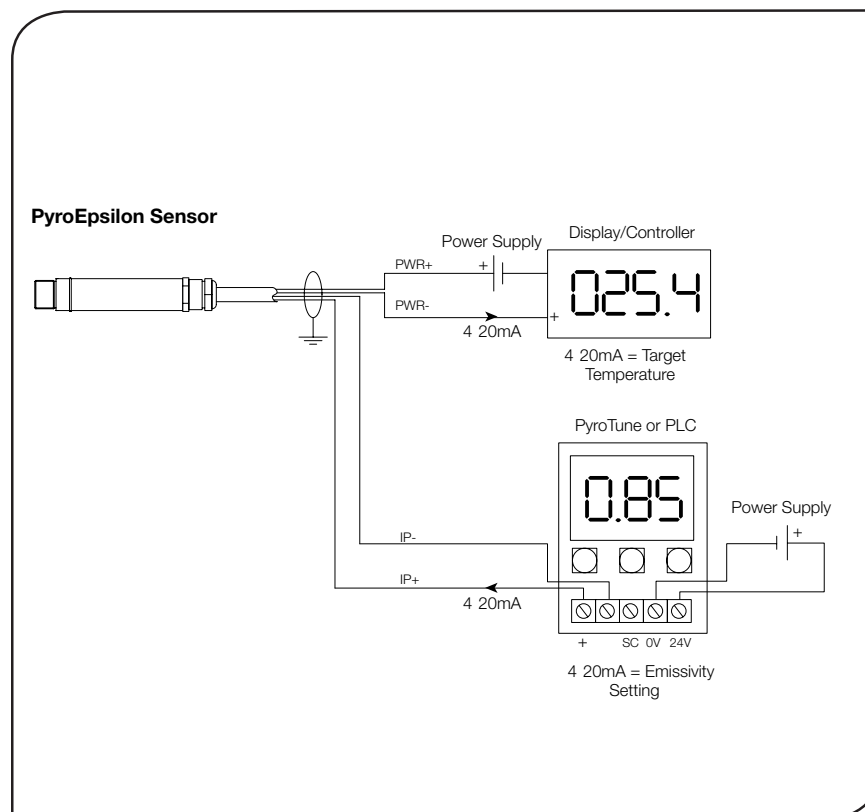
PyroEpsilon sensor with optional PyroTune emissivity adjuster
