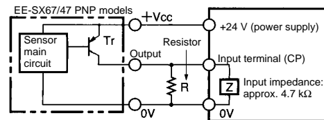
EE-SX47/67 PNP Models with a 4.7-kΩ Resistor
