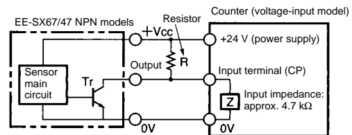
EE-SX47/67 NPN Models with a 4.7-kΩ Resistor
