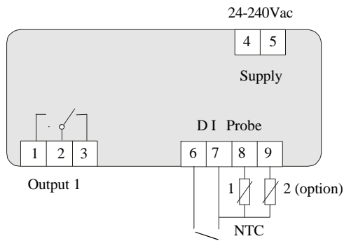
IR32 Models NTC only
