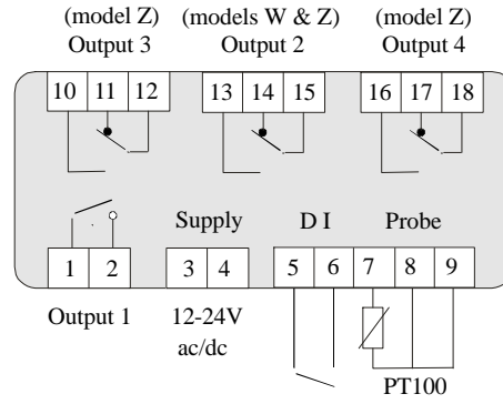
IR32V, W, Z low voltage versions
