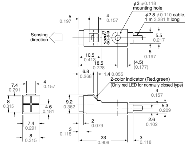
GXL-8HU type Sensor
