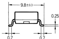
Flat Actuator Standard
