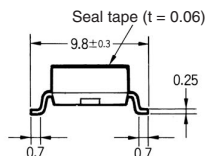
With Seal Tape
