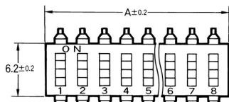
Flat Actuator Standard
