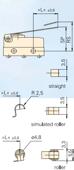
Steel auxiliary actuator
