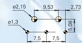
Drilling pattern for lateral PCB terminals 0.6 x 0.5, with location pins
