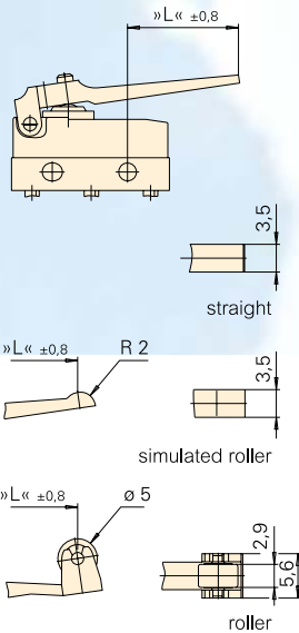
Plastic auxiliary actuator with/ without adjusting screw
