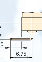
PCB terminal 0,6 x 0,5 mm LH-side w/o location pins
