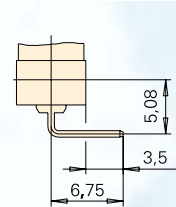
PCB terminal 0,6 x 0,5 mm RH-side w/o location pins
