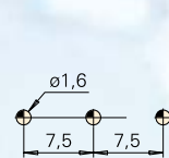
Drilling pattern for PCB terminals 1.3 x 0.5 mm
