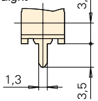
PCB terminal 0,6 x 0,5 RH-side with location pins
