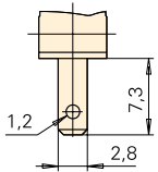
PCB terminal 0,6 x 0,5 RH-side w/o location pins
