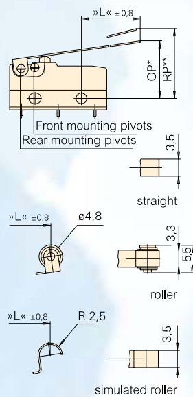
Steel auxiliary actuator
