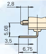
PCB terminal 0,6 x 0,5 LH-side with location pins
