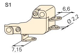
PCB terminal 1.3 x 0.8 cover side
