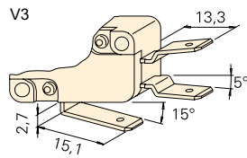
Q.C. terminal 4.8 x 0.8 dog-leg
