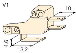
Q.C. terminal 4.8 x 0.8 straight
