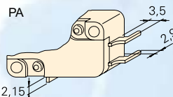
PCB terminal 1.3 x 0.8 housing side
