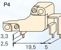
PCB terminal 1.3 x 0.5 underside
