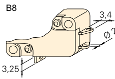
PCB terminal 1.3 x 0.8 housing side
