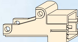
Connector housing for Q.C. terminals 6.3 x 0.8, RAST 5
