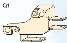
Q.C. terminal 4.8 x 0.8 straight
