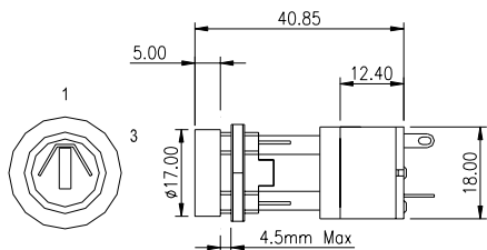
PARALLEL LOCK HEAD
