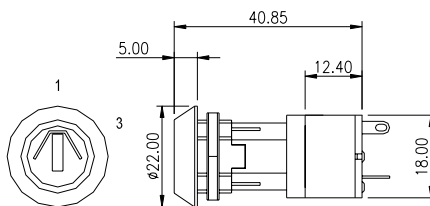
TAPERED LOCK HEAD
