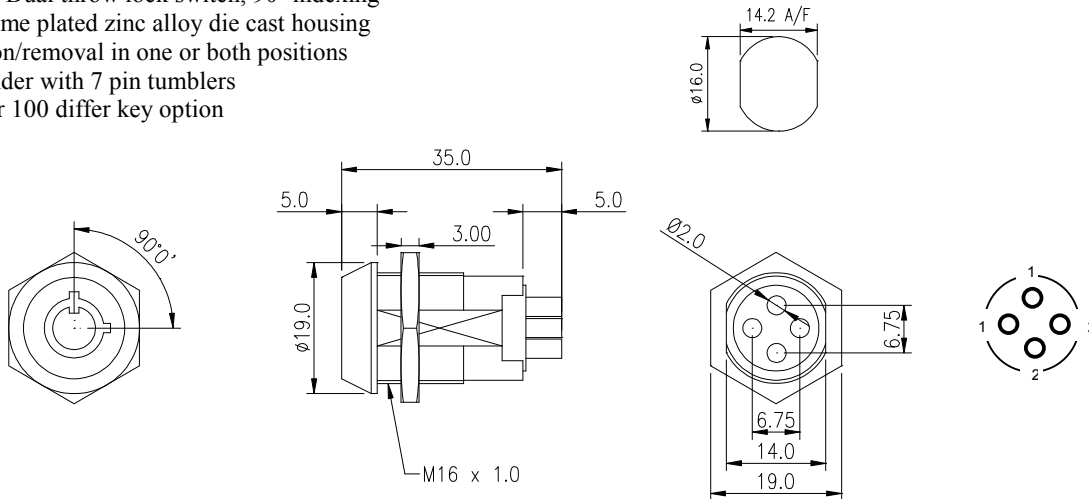
PANEL PIERCING DETAILS
