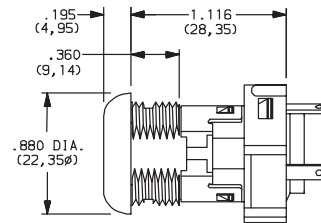
V 6 TUMBLER TUBULAR LOCK
