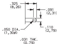
05 .110" QUICK CONNECT
