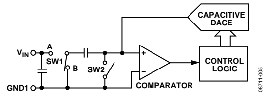
Figure 19. ADC Conversion Phase
