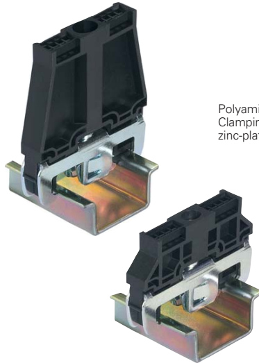
End clamp with U-foot
