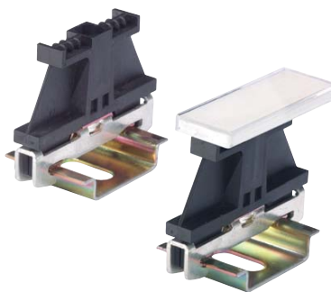
End clamp for TS 35 fixed with screw
