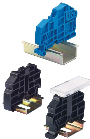
End clamp for TS 35 fixed without screw
