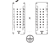
Pole assignment 16pole + ground
