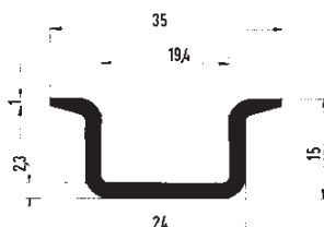
Mounting rail 35 x 15 accord. to DIN EN 60715
