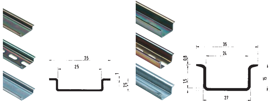
Mounting rail 35 x 7,5 according to DIN EN 60715
