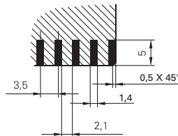
Detail Z
