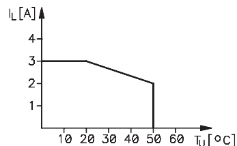
Derating curve:
