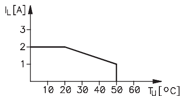
Derating of three phase contactor
