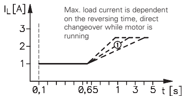
Reversing contactor in dynamic mode
