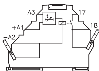
Terminal assignment: Timer relay
