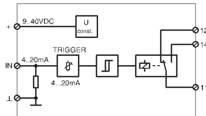
Wiring diagram Current relay SR 4...20 mA
