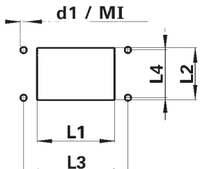
Mounting dimensions and cut-outs for open-bottom housings
