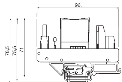
RAB – 2 Changeover contact (DPDT)
