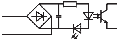
Block diagram of AC/DC input
