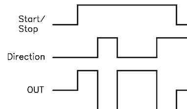
Timing diagram for DC motor-reversing contactor
