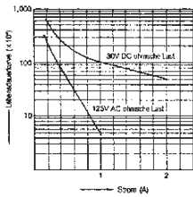
Typical endurance curve of a relay
