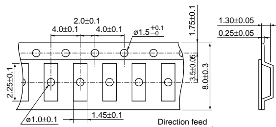
PR*21_RK Series: Embossed Tape
