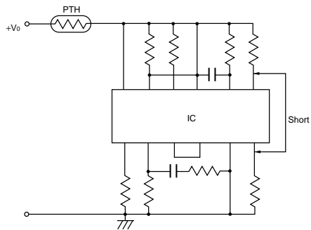
(3) Short-Circuit Test of IC
