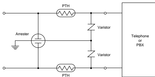
(5) Telecommunication Circuit
