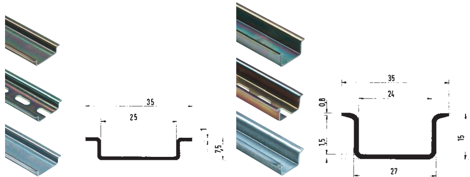
Mounting rail 35 x 7,5 according to DIN EN 60715
