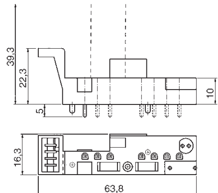
Pin base
