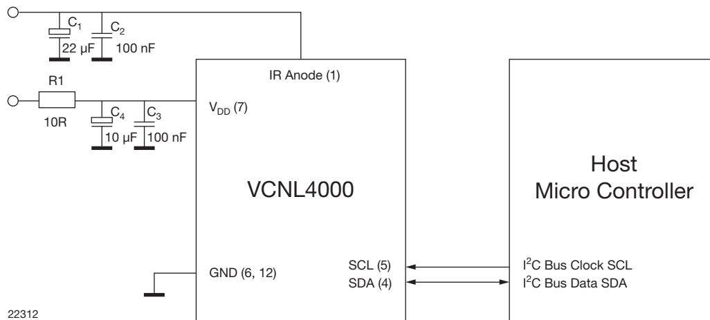
Fig. 12 - Application Circuit (x) = Pin Number
