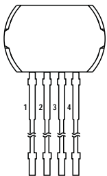
Pin-out Diagram
