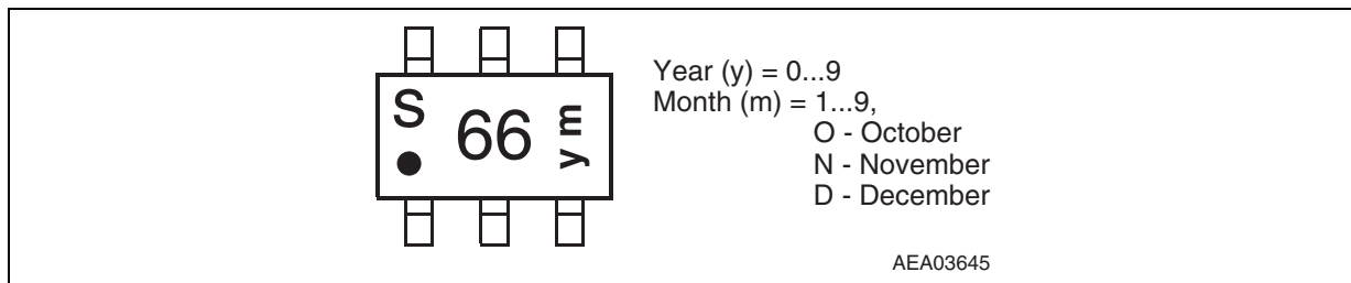
Figure 6 Marking PG-TSOP6-6-5
