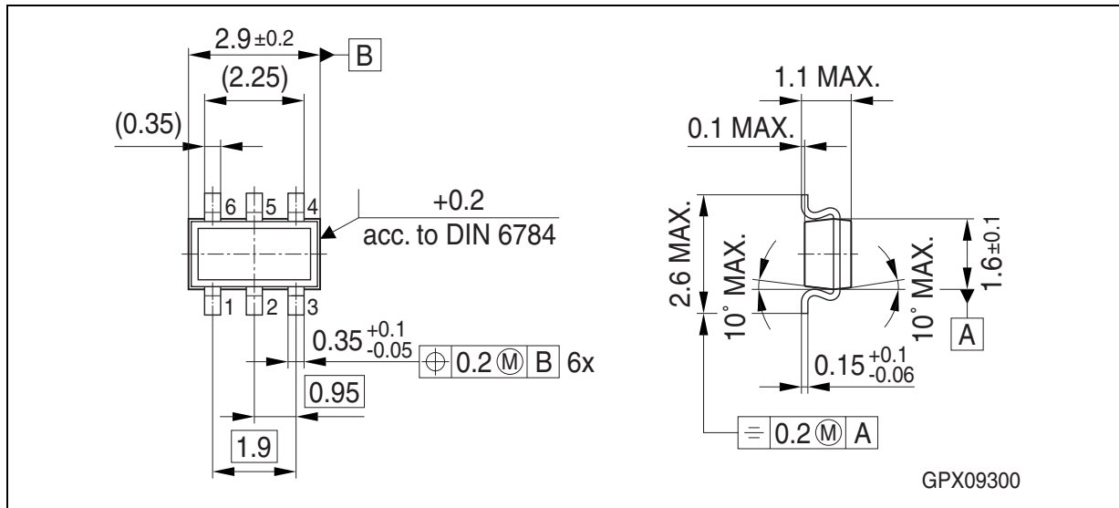
Figure 8 PG-TSOP6-6-5 (Plastic Thin Small Outline Package)
