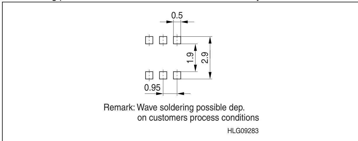
Figure 9 Footprint PG-TSOP6-6-5
