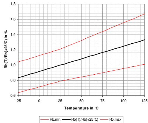
Figure 7: bridge resistance related to room temperature value
