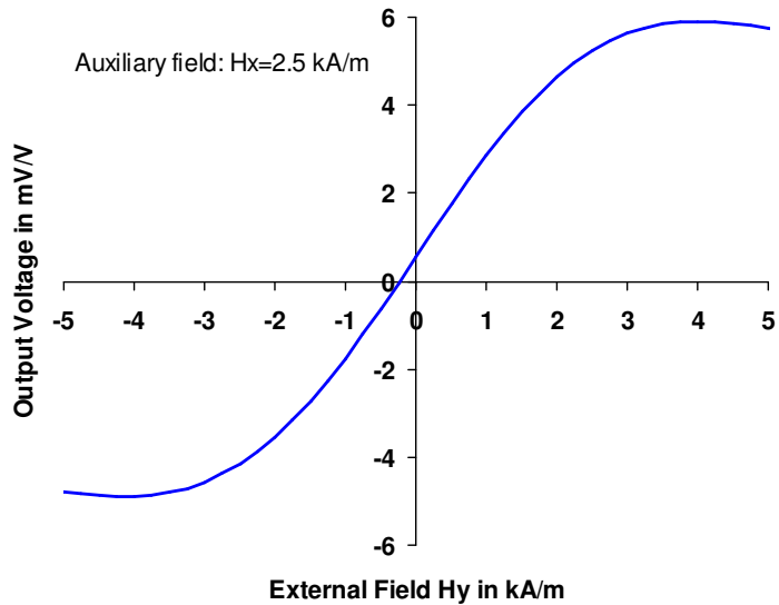
Figure 5: Characteristic curve for KMY21M
