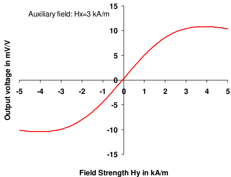
Figure 4: Characteristic output curve of KMY & KMZ for an auxiliary field strength of H_x=3 kA/m
