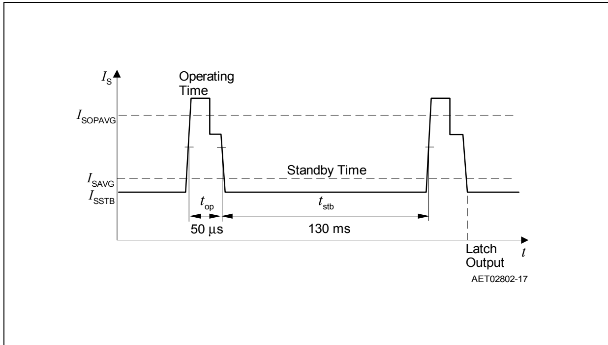
Figure 3 Timing Diagram
