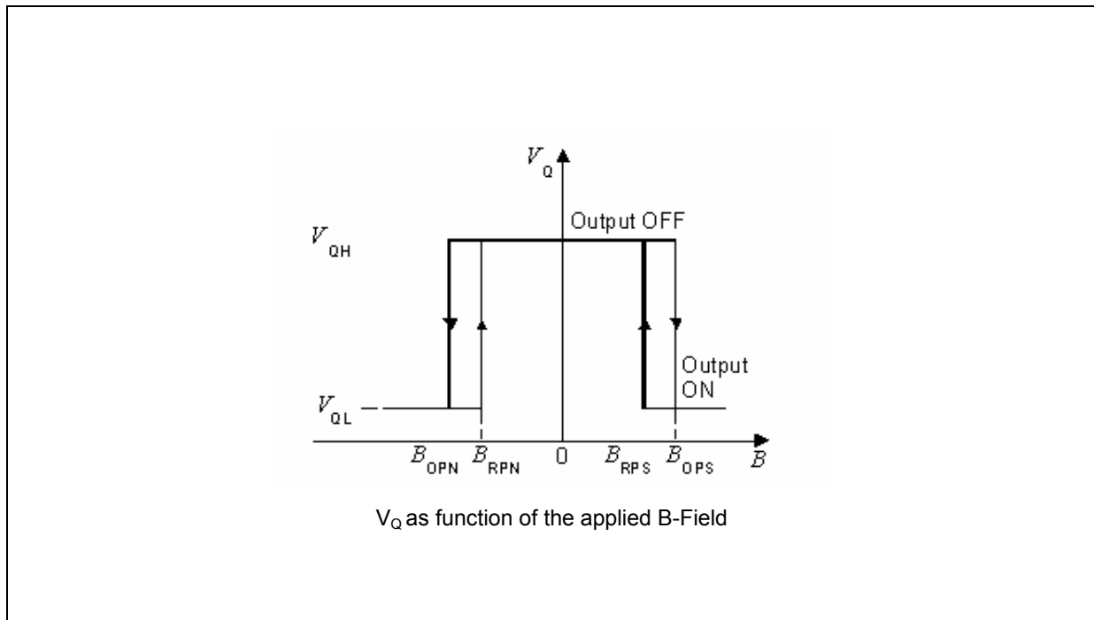
Figure 4 Output – Signal TLE 4913
