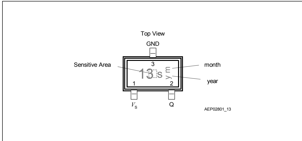
Figure 1 Pin Configuration (top view)
