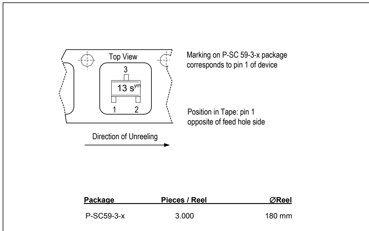
Figure 5 Marking and Tape Loading Orientation
