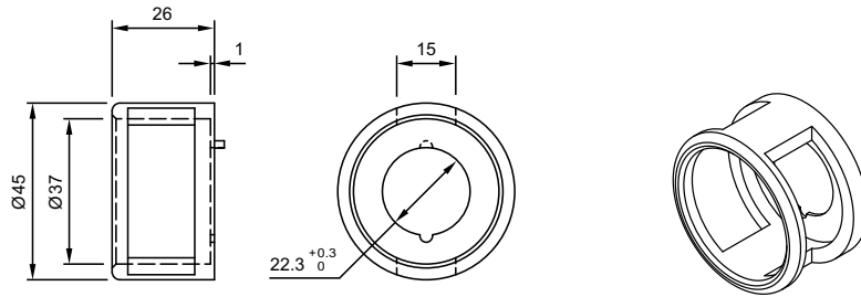
13 Mounting flange page 139
