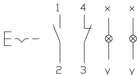
6 Illuminated pushbutton actuator triple page 38
