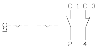
21 Keylock switch 2 positions page 39
