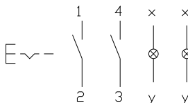
8 Illuminated pushbutton actuator double page 38
