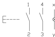
16 Illuminated pushbutton actuator double page 38
