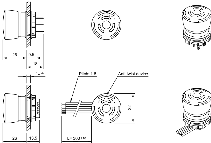
18 Illuminated pushbutton actuator page 127 | Pushbutton actuator page 128
