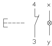
11 Illuminated pushbutton actuator single page 37
