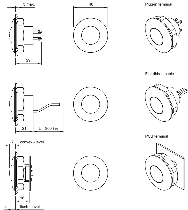
18 Illuminated pushbutton actuator page 127 | Pushbutton actuator page 128
