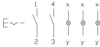
10 Illuminated pushbutton actuator single page 37
