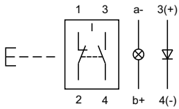
55 Illuminated pushbutton actuator page 8
