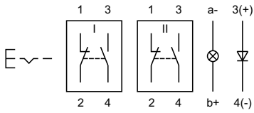
5 Illuminated pushbutton actuator page 8
