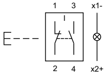
54 Illuminated pushbutton actuator page 8
