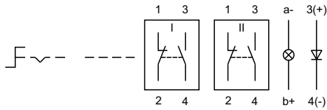
23 Selector switch 2 positions page 11
