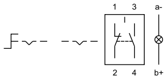
40 Selector switch 2 positions page 11
