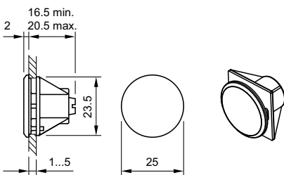
11 Blind plug, flush mounting page 27
