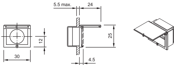
9 Protective cover, flush mounting page 27
