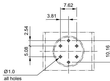
PCB layout (conductor side)
