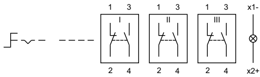
22 Selector switch 2 positions page 11
