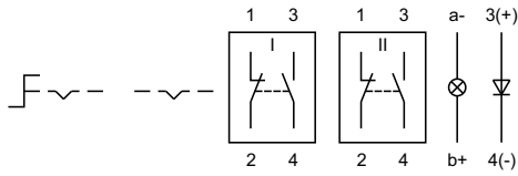
37 Selector switch 2 positions page 11
