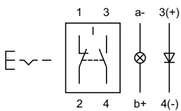
9 Illuminated pushbutton actuator page 8
