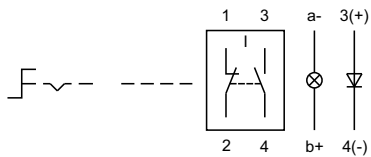
27 Selector switch 2 positions page 11
