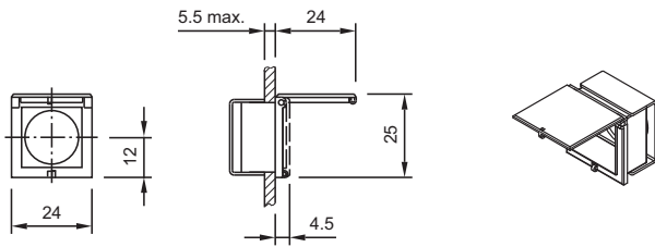
8 Protective cover, flush mounting page 27
