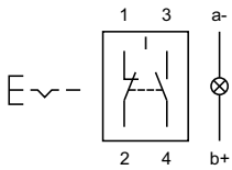
8 Illuminated pushbutton actuator page 8
