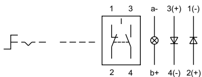
27 Selector switch 2 positions page 11
