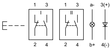
51 Illuminated pushbutton actuator page 8
