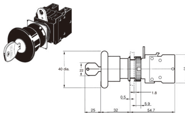
A22E-MK Medium Push-lock, Key-reset (40-dia.)
