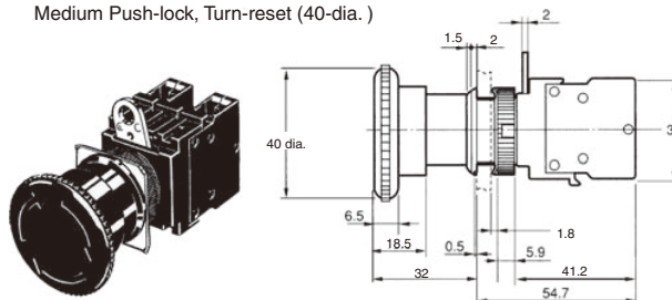
A22E-M Medium Push-lock, Turn-reset (40-dia.)
