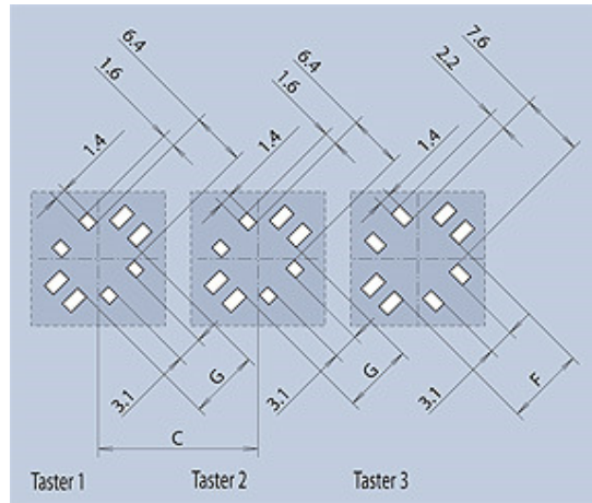
Layoutvorschlag · Layout Suggestion
