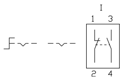
24 Selector switch 2 positions page 12 | Selector switch actuator 2 positions, flush mounting page 16
