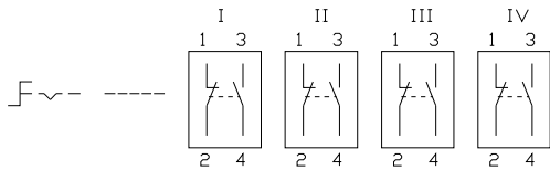
21 Selector switch 2 positions page 12 | Selector switch actuator 2 positions, flush mounting page 16
