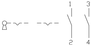
55 Keylock switch 2 positions page 11 | Keylock switch actuator 2 positions, flush mounting page 15
