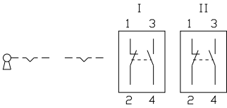
52 Keylock switch 2 positions page 11 | Keylock switch actuator 2 positions, flush mounting page 15
