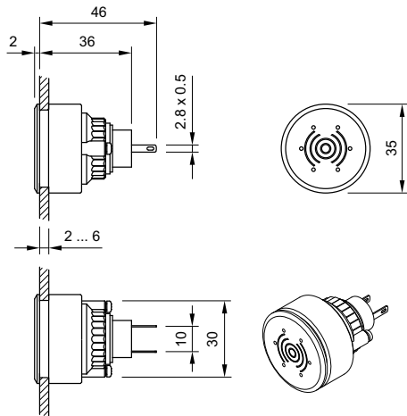
17 Indicator actuator full face illumination page 6
