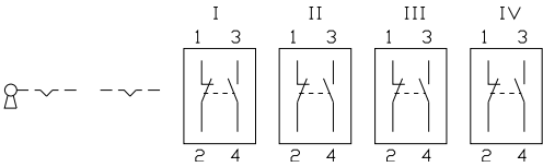
54 Keylock switch 2 positions page 11 | Keylock switch actuator 2 positions, flush mounting page 15
