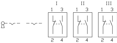
53 Keylock switch 2 positions page 11 | Keylock switch actuator 2 positions, flush mounting page 15
