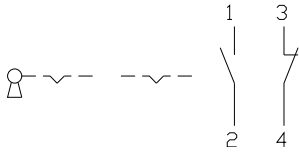
55 Keylock switch 2 positions page 11 | Keylock switch actuator 2 positions, flush mounting page 15
