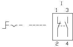
18 Selector switch 2 positions page 12 | Selector switch actuator 2 positions, flush mounting page 16
