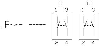
19 Selector switch 2 positions page 12 | Selector switch actuator 2 positions, flush mounting page 16
