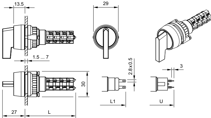
23 Selector switch 2 positions page 12
