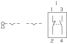
51 Keylock switch 2 positions page 11 | Keylock switch actuator 2 positions, flush mounting page 15
