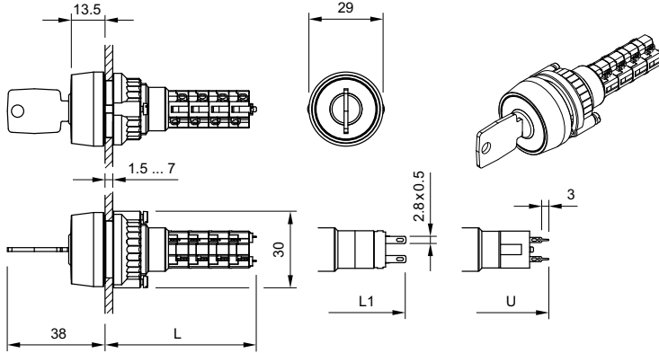
22 Selector switch 2 positions page 12
