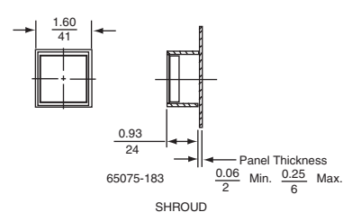
Shroud
