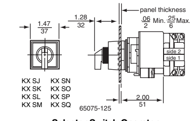
Selector Switch Operator Illuminated
