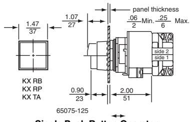
Single Push Button Operator Illuminated
