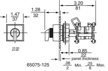
Double Pot Potentiometer Operator
