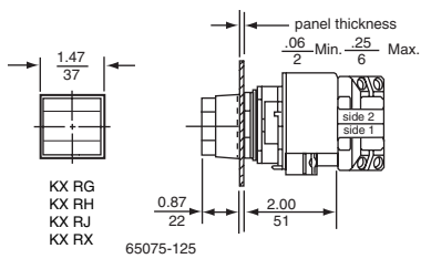
Dual Push Button Operator Illuminated
