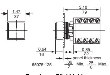
Four Lamp Pilot Light
