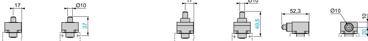
(1) 1 tapped entry for ISO M20 x 1.5 or Pg 13 cable gland or 1/2" NPT. Ø: 2 elongated holes Ø 5.3 x 7.3.
