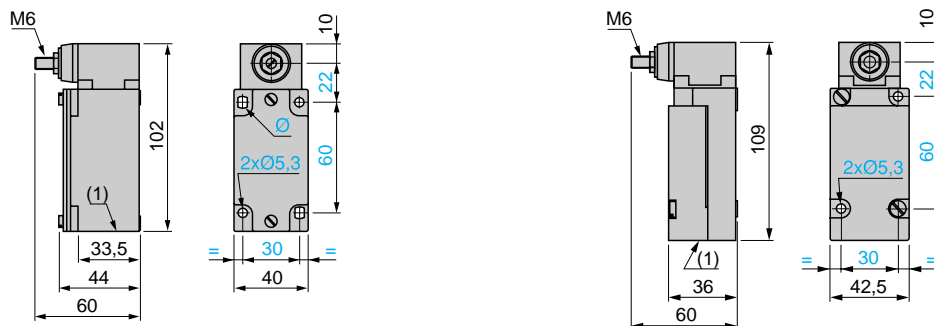
(1) 1 tapped entry for ISO M20 x 1.5 or Pg 13 cable gland or 1/2" NPT. Ø: 2 elongated holes Ø 5.3 x 7.3.
