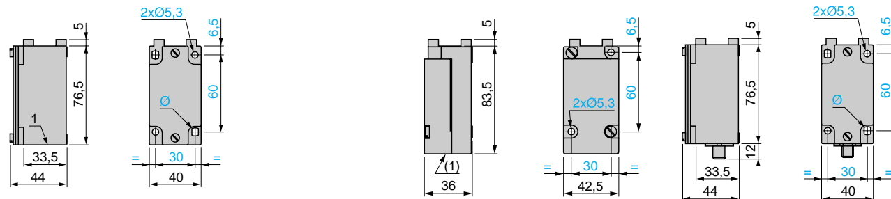
(1) 1 tapped entry for ISO M20 x 1.5 or Pg 13 or cable gland or 1/2" NPT. Ø: 2 elongated holes Ø 5.3 x 7.3.
