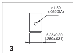
Quick-connect
