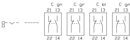
30 keylock switch 2 positions 45 - 70 mm, keylock switch 2 positions for flush mounting 51 - 79 mm page 598, 612
