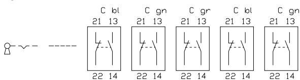
31 keylock switch 2 positions 45 - 70 mm, keylock switch 2 positions for flush mounting 51 - 79 mm page 598, 612
