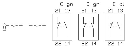
27 keylock switch 2 positions 45 - 70 mm, keylock switch 2 positions for flush mounting 51 - 79 mm page 598, 612
