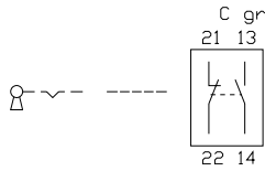
26 keylock switch 2 positions 45 - 70 mm, keylock switch 2 positions for flush mounting 51 - 79 mm page 598, 612
