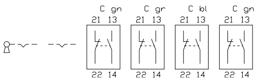
29 keylock switch 2 positions 45 - 70 mm, keylock switch 2 positions for flush mounting 51 - 79 mm page 598, 612
