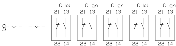
31 keylock switch 2 positions 45 - 70 mm, keylock switch 2 positions for flush mounting 51 - 79 mm page 598, 612
