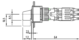
55 selector switch 2 positions for flush mounting 51 - 79 mm page 617
