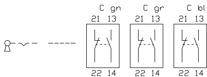
28 keylock switch 2 positions 45 - 70 mm, keylock switch 2 positions for flush mounting 51 - 79 mm page 598, 612
