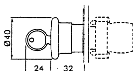
ZB2-BS14 (1)
