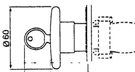
ZB2-BS24 (1)
