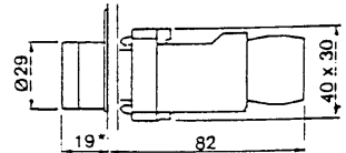
XB2-BW3 (with transformer) ZB2-BW1●, BW3●, ZB2-BK●●●(1) ZB2-BW03●, BW04●, BW093●(2)
