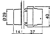
XB2-BV6● ZB2-BV0●(1) ZB2-BV6 (2)
