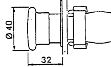
XB2-BC●● ZB2-BC● and BT●(1)
