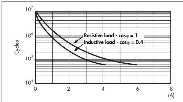
F 34 - Electrical life (AC) v contact current
