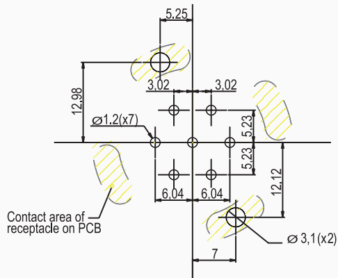
DRILLING PATTERN
