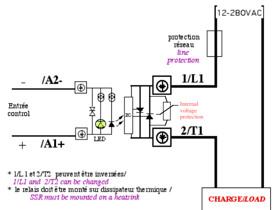
SUL842070= SU842070 SSR + WF311100 heatsink (*) 20A AC-51 see derating curve
