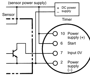
Operates with NPN transistor ON
