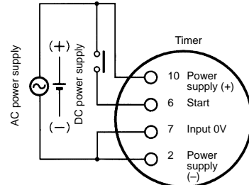
Operates with relay ON
