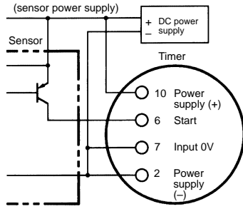
Operates with PNP transistor ON
