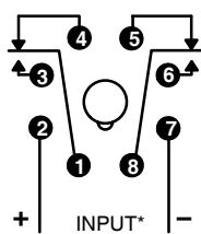
DPDT, 2 Form "C" (8-Pin Type)
