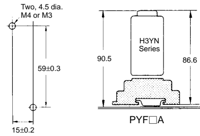
Mounting Holes
