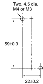
Mounting Holes
