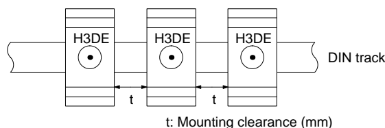
t: Mounting clearance (mm)
