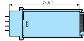
Spring clip for PCB base 26 532 704
