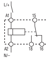
Wiring diagram (without signal START)
