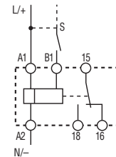
Wiring diagram (with signal START)
