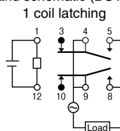
Pin layout and schematic (BOTTOM VIEW)
