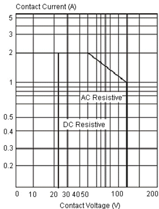
Maximum Switching Power
