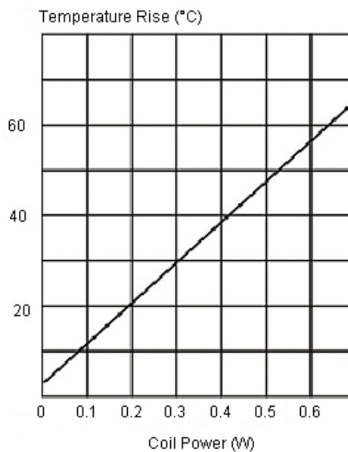
Coil Temperature Rise
