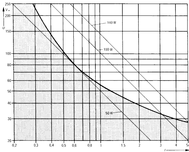
Load limit curve for contact sets F1xx
