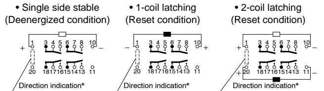
Schematic (Bottom view)
