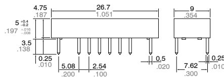
Standard PC board terminal
