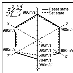
12.-(2) Malfunctional shock (latching) Tested sample: TQ2-L-12V, 6 pcs.
