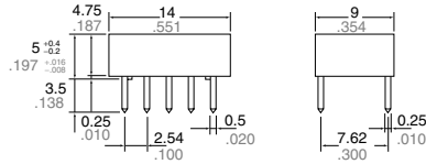
Standard PC board terminal
