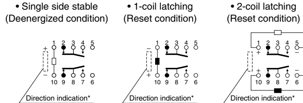
Schematic (Bottom view)
