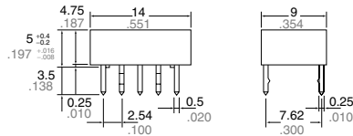
Self-clinching terminal
