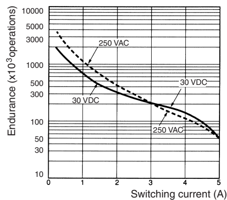
MY4 (Resistive Loads)
