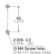
Panel cutout
