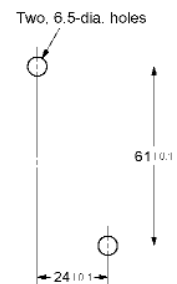
Mounting Hole Dimensions (TOP VIEW)
