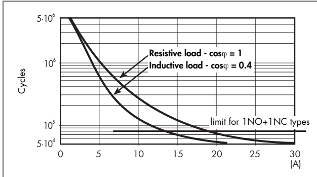
F 65 - Electrical life (AC) v contact current
